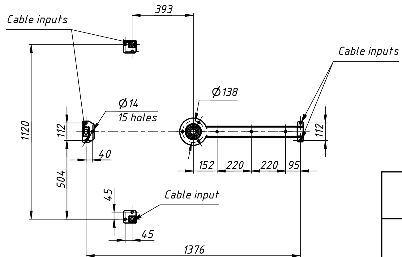
Instalation tamplate
