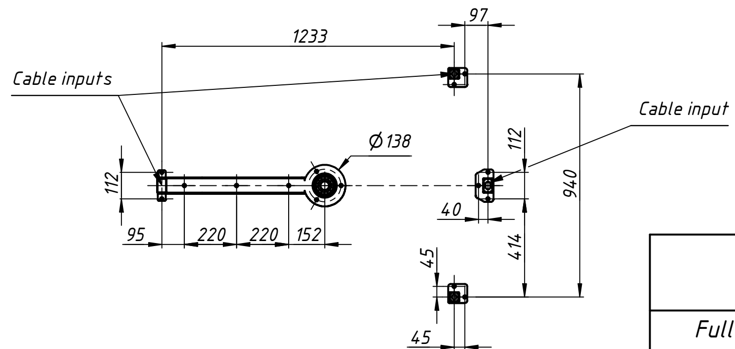
Installation template
