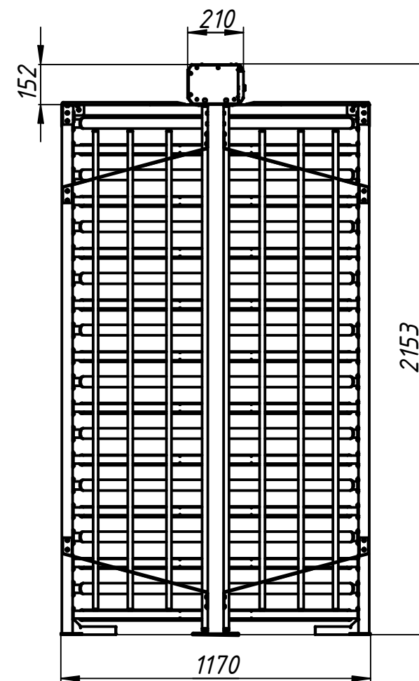
Instalation tamplate
