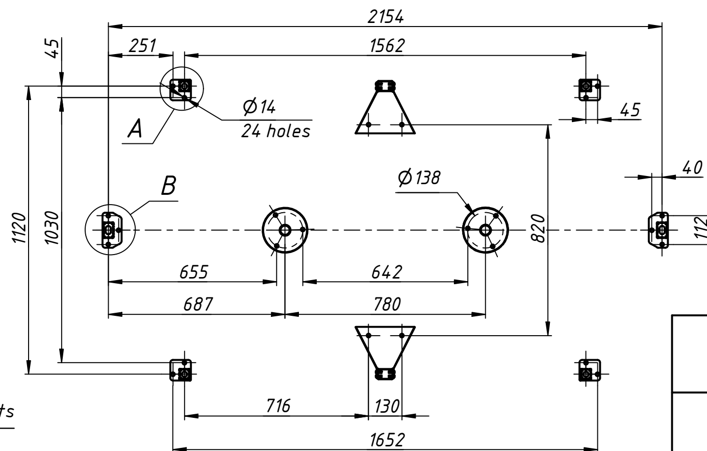
Instalation tamplate
