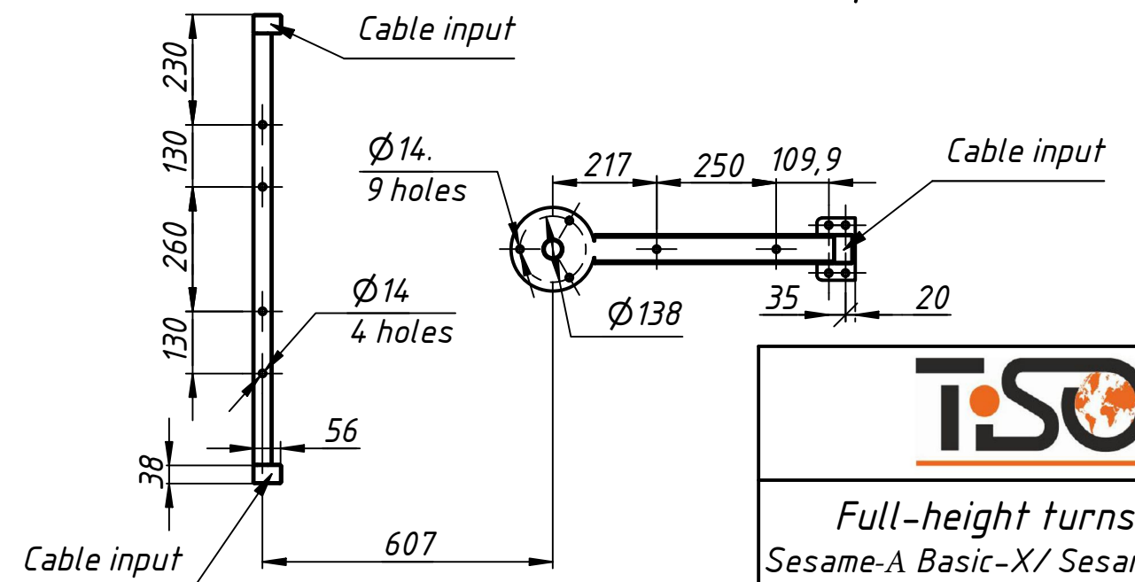
Installation tamplate
