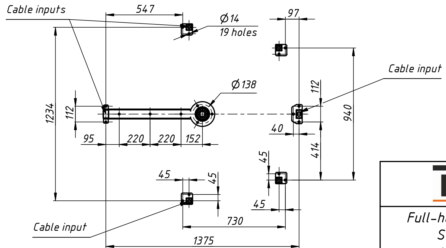
Installation template
